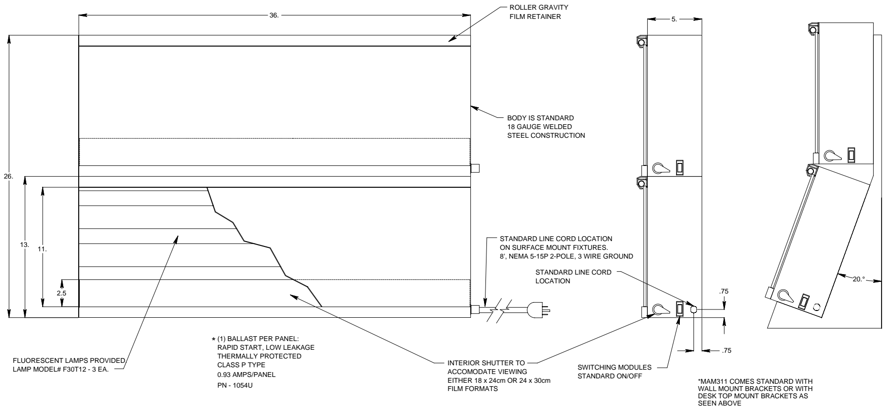
FRONT VIEW
