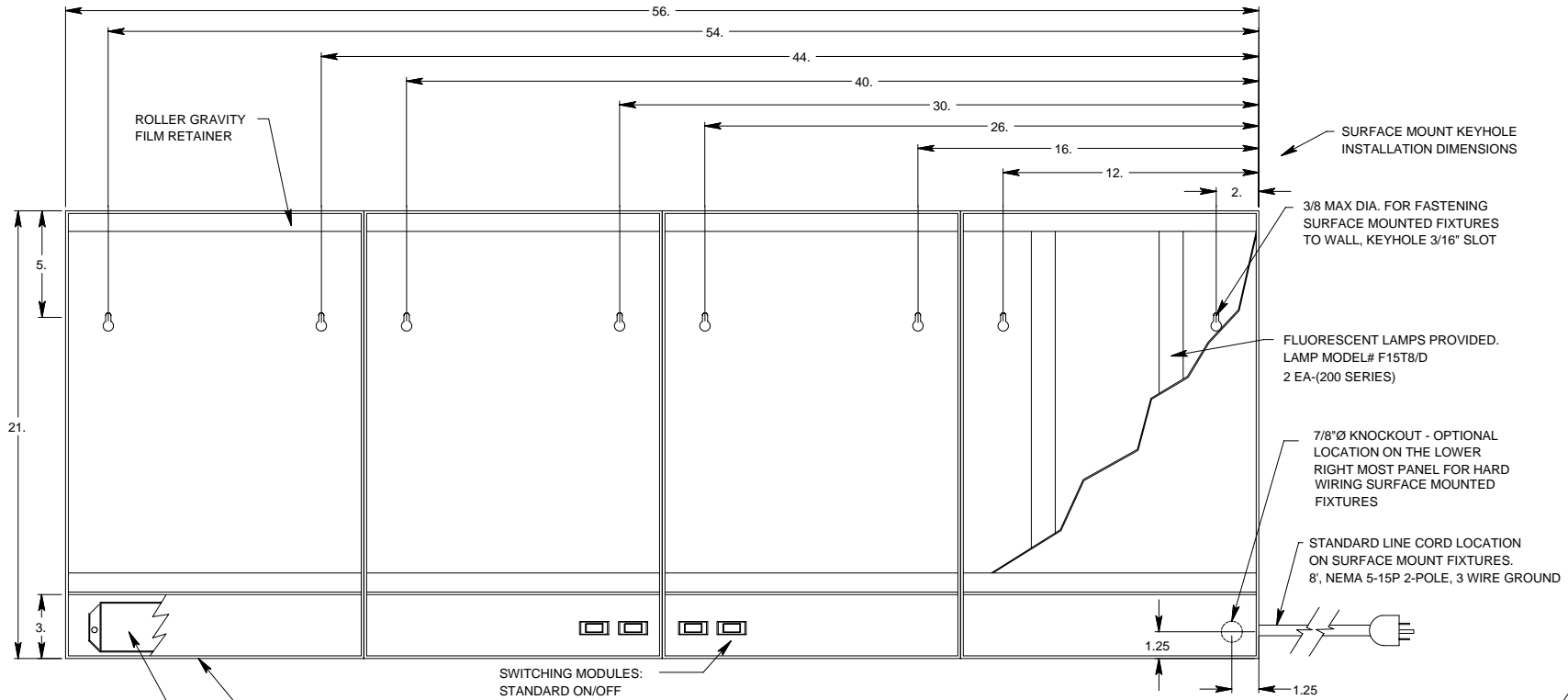
FRONT VIEW
